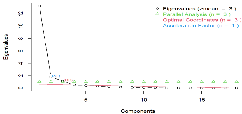
Fig.1. Scree plot.
