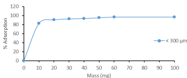
Figure 1: Effect of MRC-CNTs weight on % adsorption of 50 ppm of \text{Pb}^{2+} ions.
