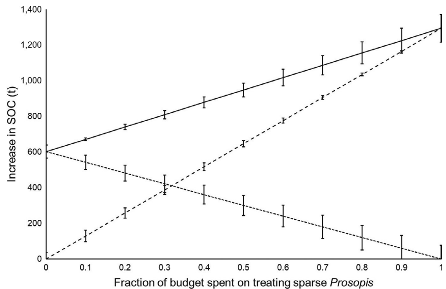
FIGURE 2 Estimated increase in SOC (average of nine sublocations) following Prosopis removal and grassland restoration, as a function of the fraction of the budget spent on treating Ps and Pd (long and short dashes, respectively). The solid line indicates the combined increase. Error bars indicate one Standard Error
