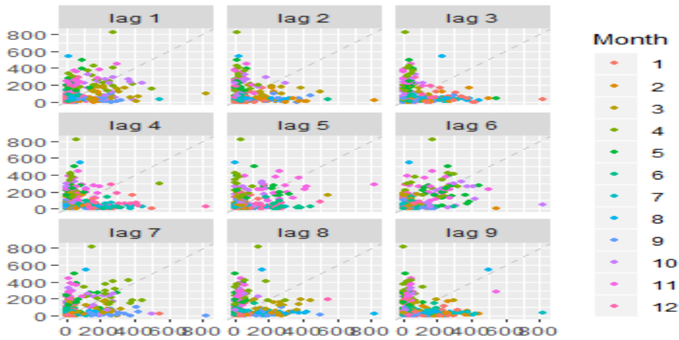
Fig. 4. Scatter plot at various lags
