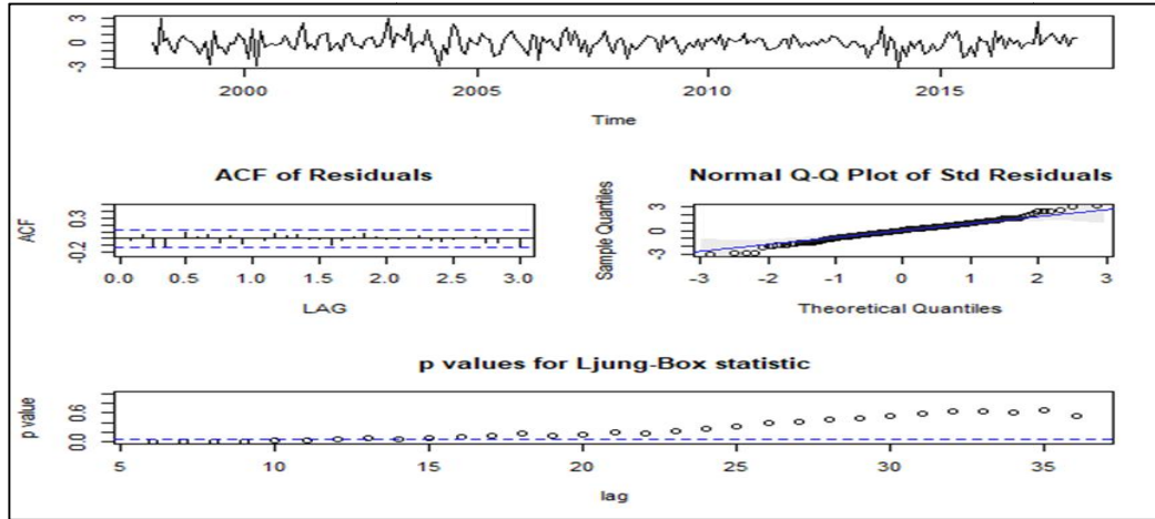
Fig. 5. Diagnostic Analysis: Residuals for SARIMA (1, 1, 1), (0, 1, 2) 12 model for the Embu county Rainfall data
