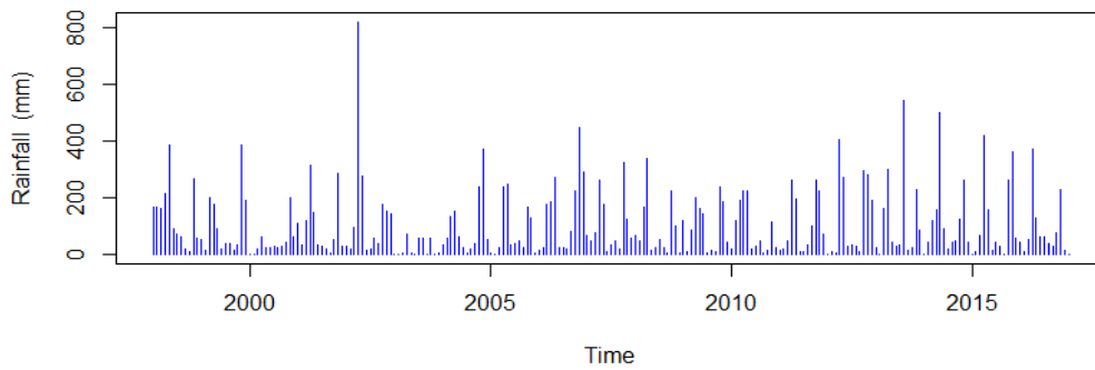
Fig. 2. Plot of monthly-time rainfall data
